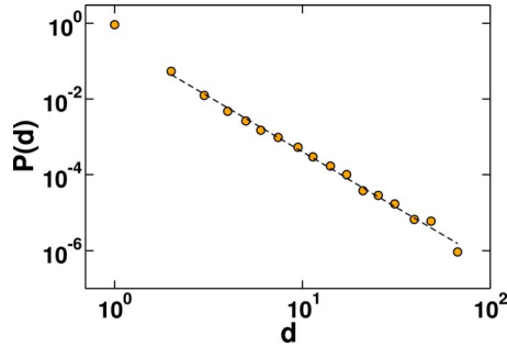
FIG. 8. (Color online) We consider only the IDs of authors with full version of their first names. Then, we count the number of times d the same ID is obtained from authors with different first names (plus middle names, if present). The probability P(d) (plotted as yellow circles) of finding an ID with “degeneracy” in the first name equal to d has a power law decay as d increases (the dashed line has exponent equal approximately to -3 ).
