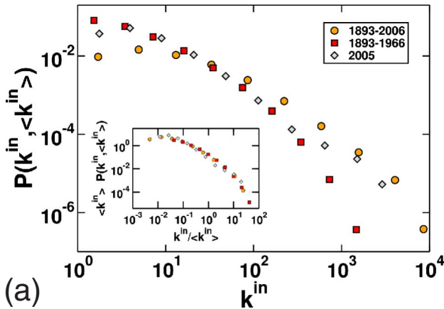
FIG. 4. (Color online) Probability densities for the indegree (a) and the instrength (b). Calculations have been performed on different WACNs based on papers published in different periods of time (yellow circles, 1893–2006; red squares, 1893–1966; and gray diamonds 2005). The insets show the same distribution as in the main plots, but opportunely rescaled by their average values.
