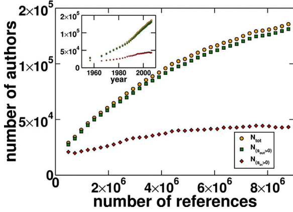
FIG. 3. (Color online) In the main plot, the total number of authors N_{tot} (yellow circles), number of authors with outstrength larger than zero N_{(s^{out}>0)} = \sum_j \theta(s_j^{out}) (green squares) and number of authors with instrength larger than zero N_{(s^{in}>0)} = \sum_j \theta(s_j^{in}) (red diamonds) are plotted as functions of the number of references (referenced papers), where \theta(\cdot) is the step function equal to one when its argument is larger than zero and null otherwise. In the inset the same quantities as those of the main plot are considered, but now they are plotted as functions of time. More specifically, each x value corresponds to the average publication year of papers belonging to the respective dynamical slice of the main plot.
