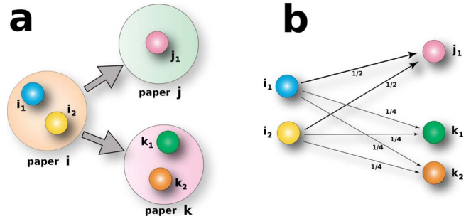
FIG. 1. (Color online) Projection of the PCN into a WACN. (a) In the network of citations between papers, the article i , written by two authors i_1 and i_2 , cites two papers j and k , written by one author j_1 and two co-authors k_1 and k_2 , respectively. (b) The WACN is then simply generated by connecting with a directed link both i_1 and i_2 to j_1 , each with weight of 1/2 , and to k_1 and k_2 , each with weight of 1/4 .
