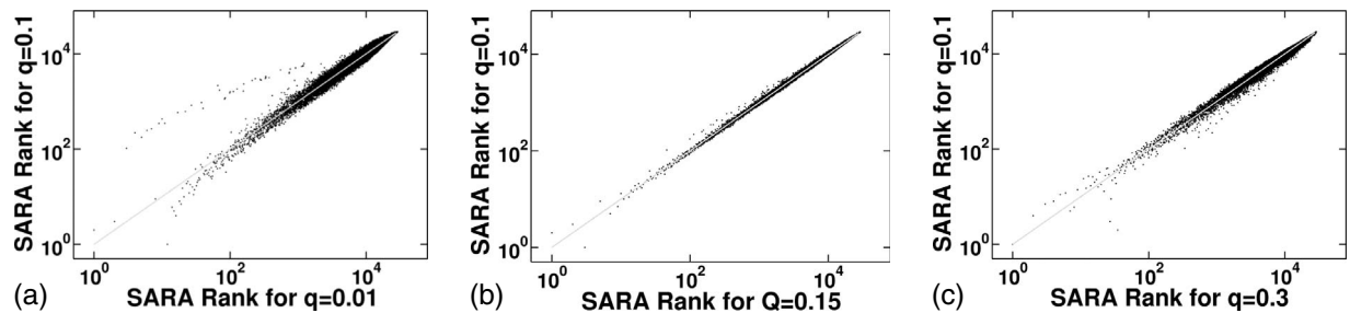
FIG. 9. The rankings calculated with SARA for q=0.1 are plotted as function of the rankings obtained with the same algorithm but for different values of q : (a) q=0.01 , (b) q=0.15 and (c) q=0.3 . All plots have been generated from the WACN based on all papers published between 1893 and 1966 [the same data set as the one used in Figs. 6(a) and 6(c) of the main text].
